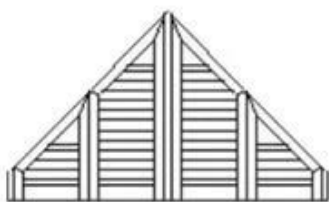
Triangular window
